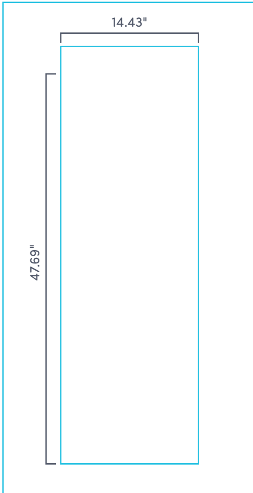
Wall cutout
