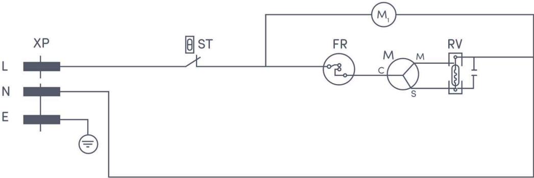
XP:inlets ST:thermostat RV:starter M:compressor FR:overload protector M1:fan
