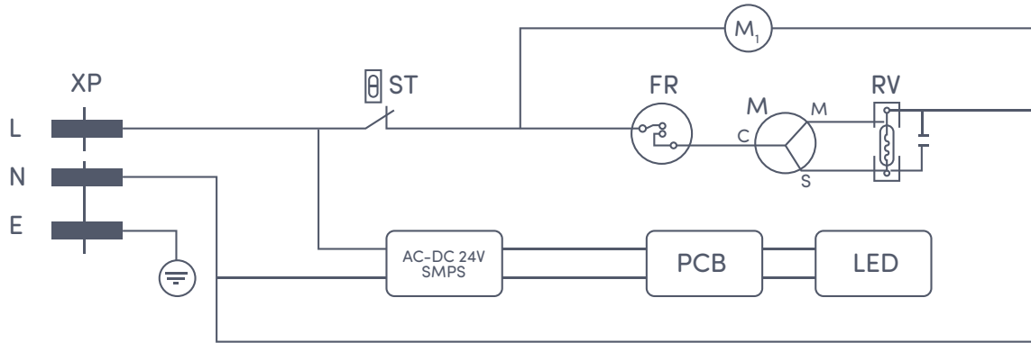
XP:inlets ST:thermostat RV:starter M:compressor FR:overload protector M1:fan
