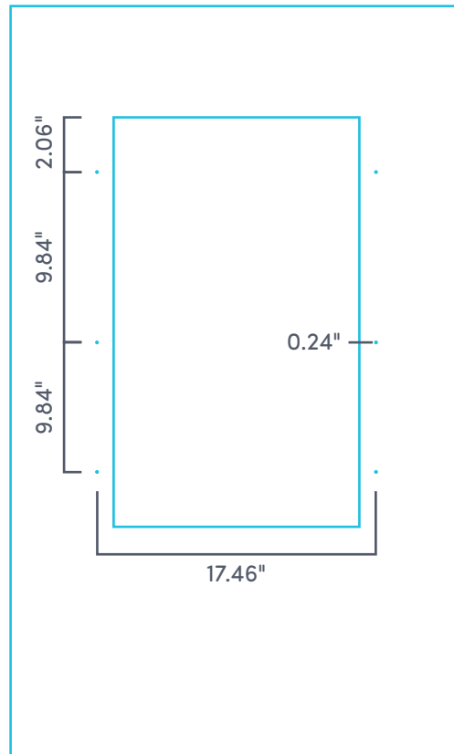
Screw holes
