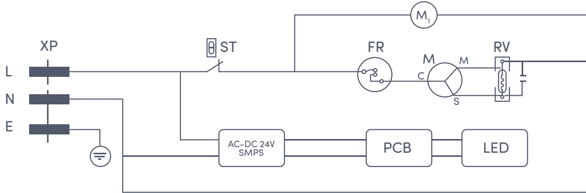
XP:inlets ST:thermostat RV:starter M:compressor FR:overload protector M1:fan
